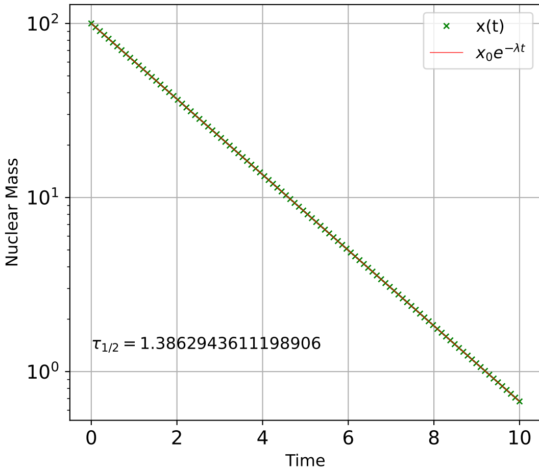
Nuclear decay curve ( \lambda = 0.5 )
