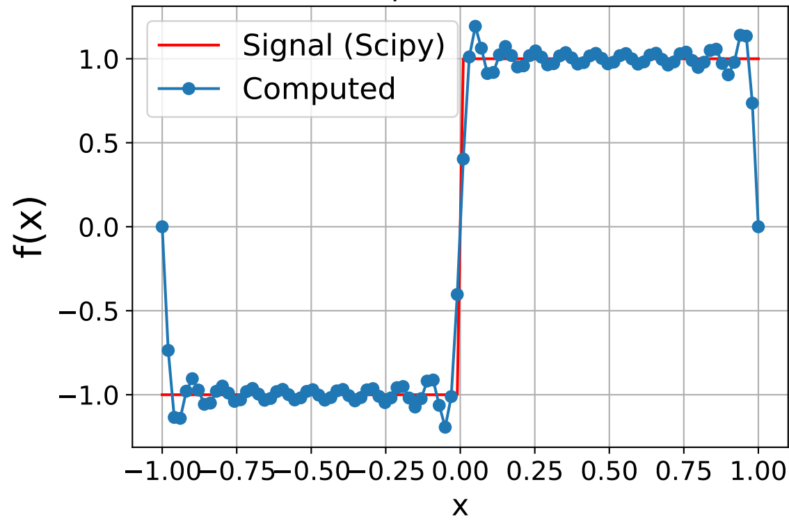
Square Wave
