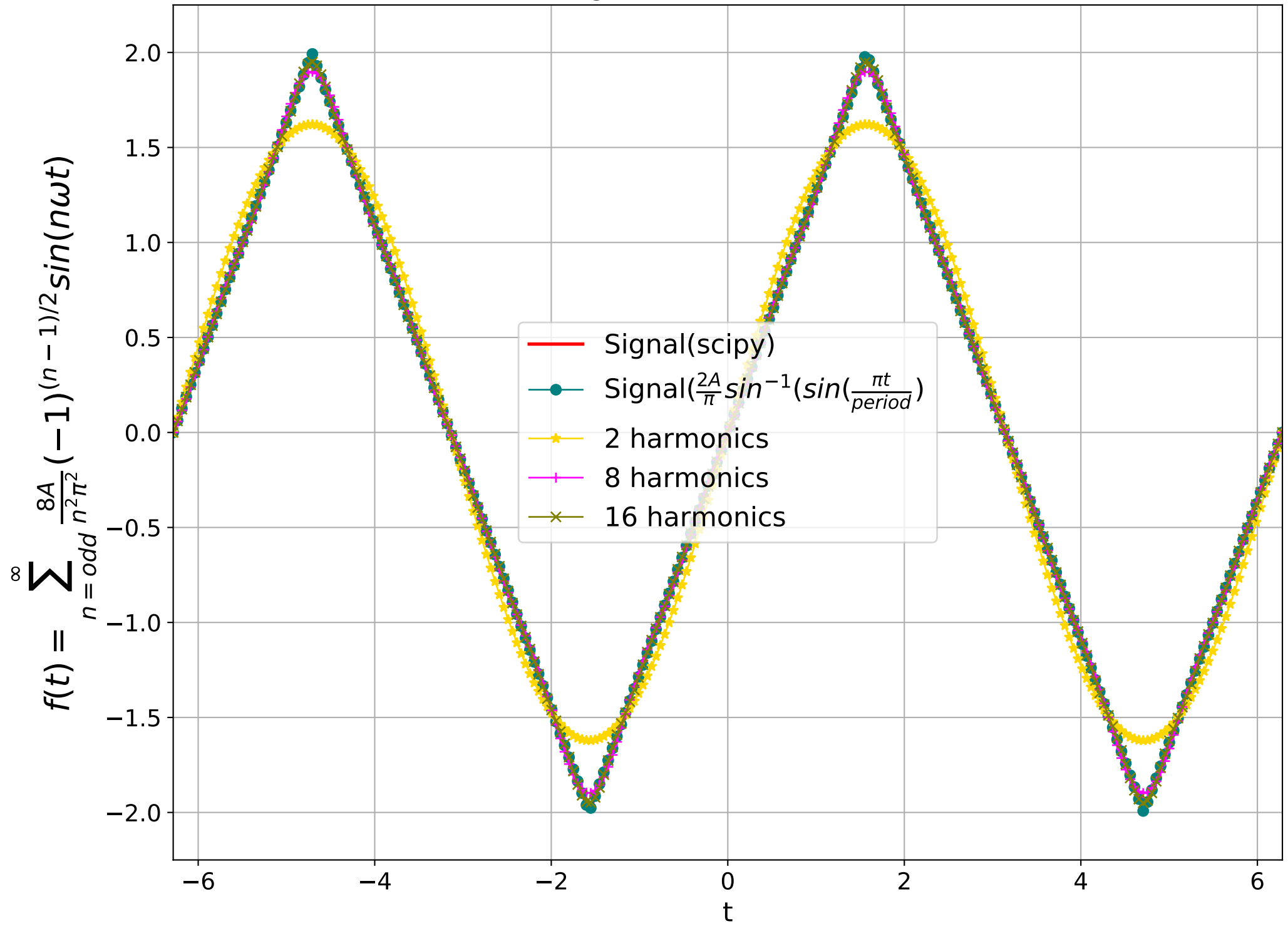
Triangular Wave Fourier Series
