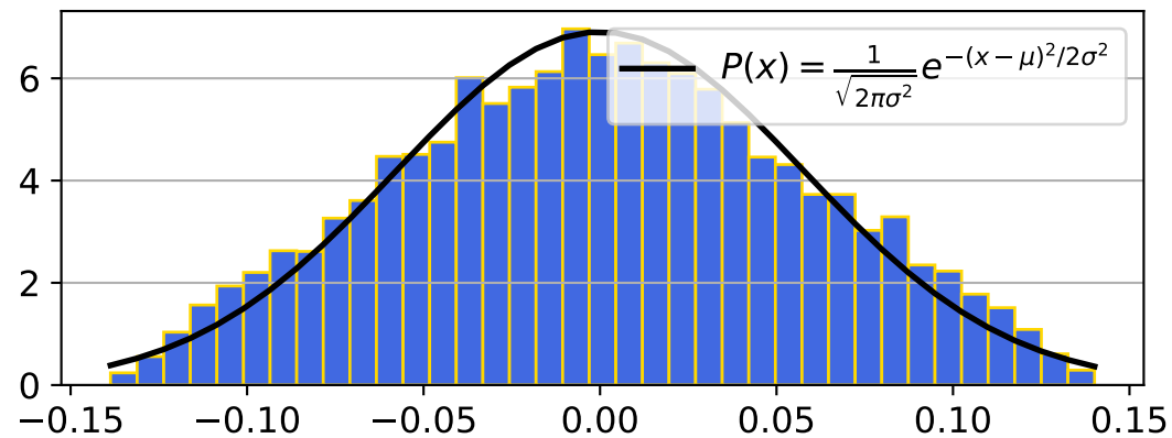
Sum of 2 Variables ( \mu = 0, \sigma = 0.05773502691896258 )
