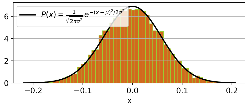
Sum of 100 Variables
