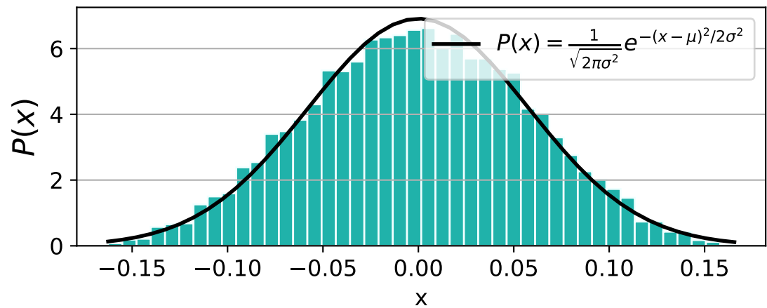
Sum of 3 Variables
