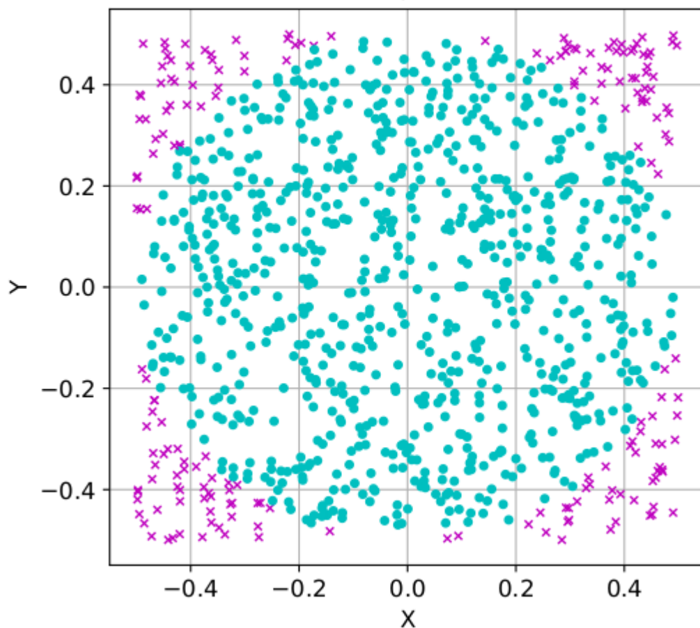
N = 1000, \pi = 3.204
