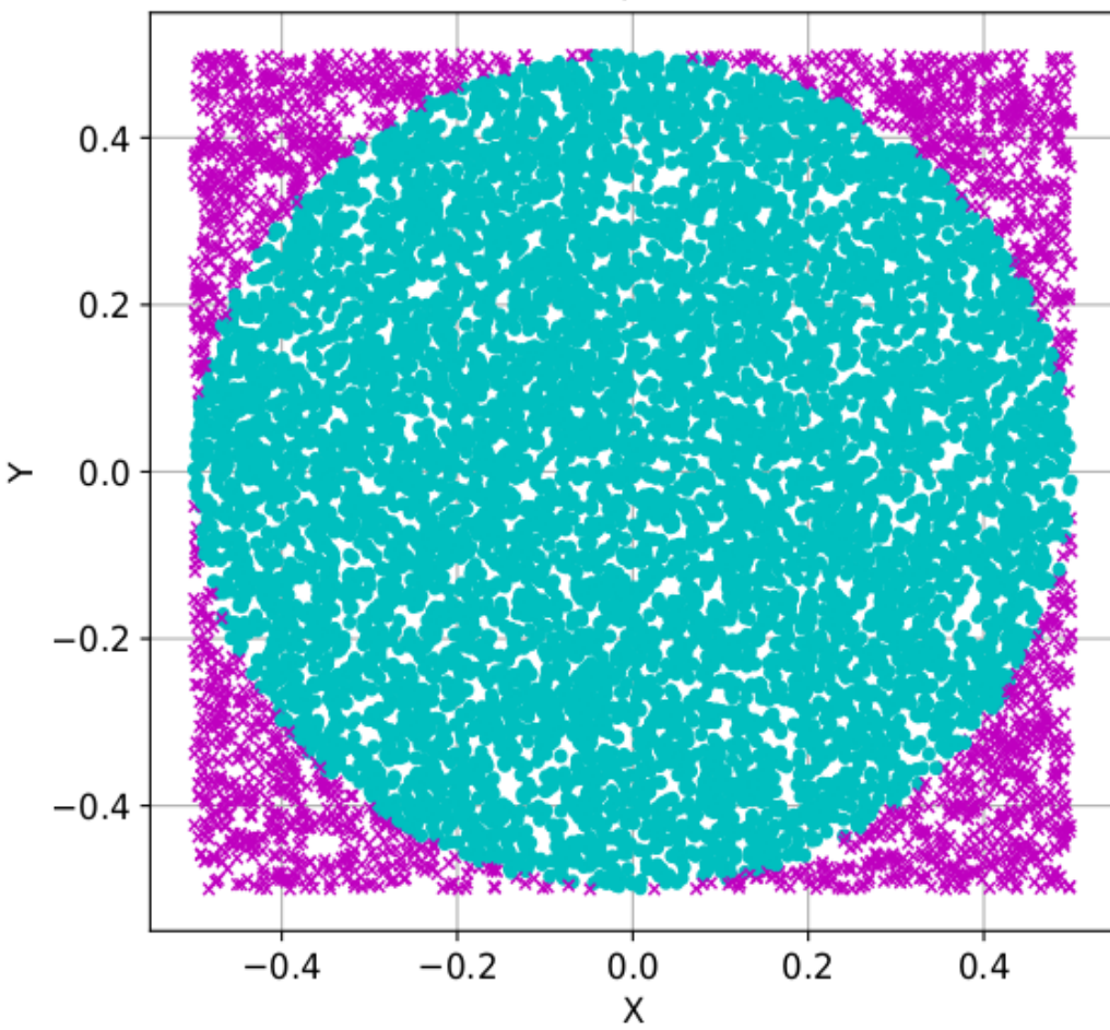
N = 10000, \pi = 3.1628
