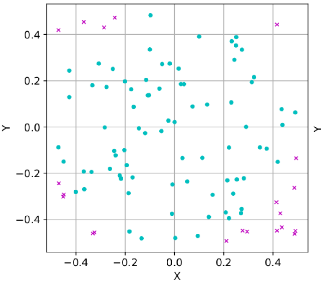
N = 100, \pi = 3.16
