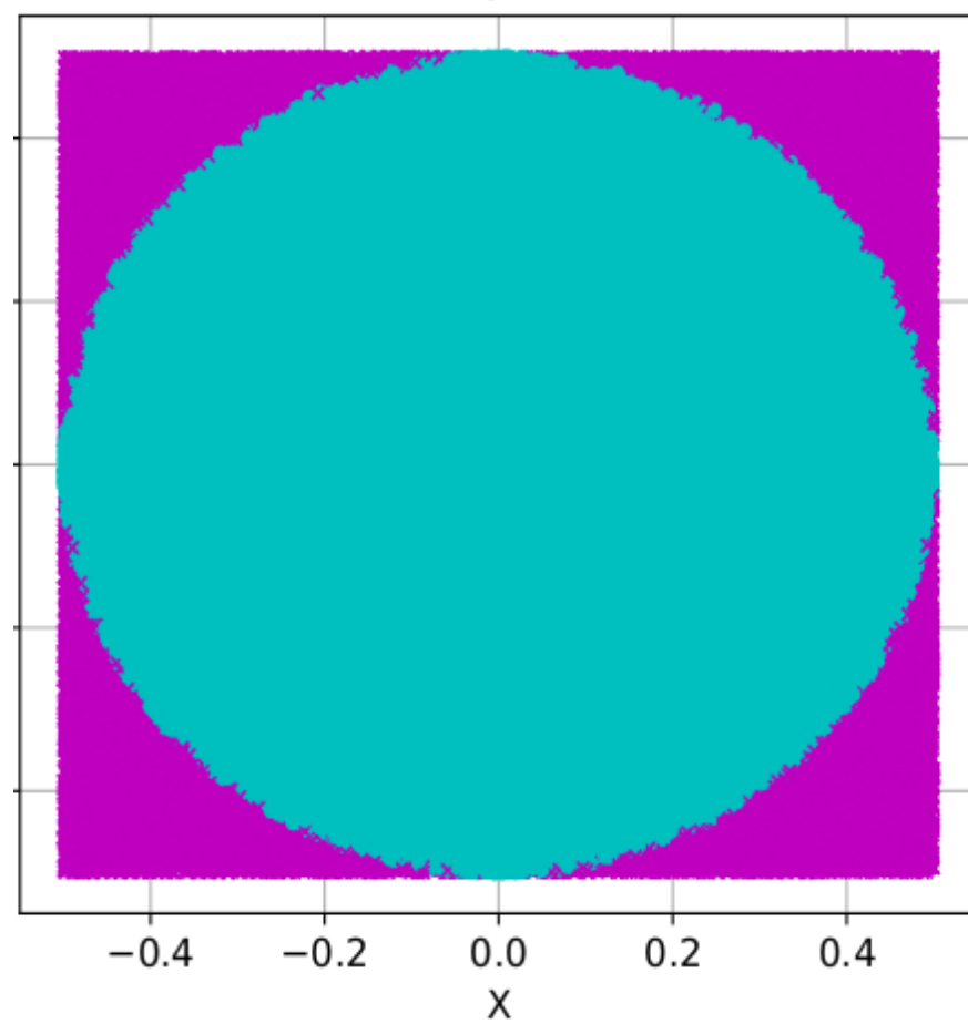
N = 100000, \pi = 3.13648
